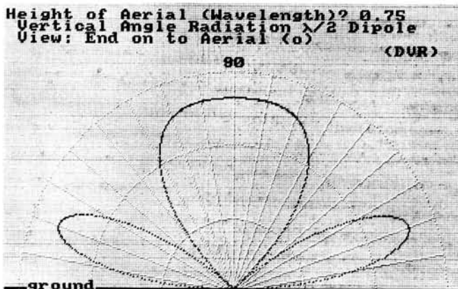
Fig. 1.7: Vertical angle radiation. Half-wave dipole at a height above ground of 0.75 wavelength. A height to be avoided at the higher frequencies
