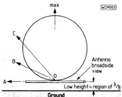
Fig. 1.3: Useful angles of radiation in the vertical mode relative to low height of antenna (text provides further explanation)
