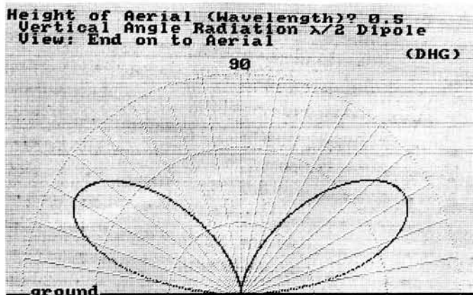
Fig. 1.6: Vertical angle radiation of a half-wave dipole at a height above ground of 0.5 wavelength. A reasonable height for say 14 and 21MHz with main lobe angles in region of 30°
