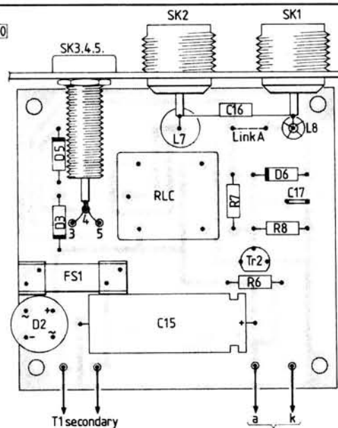
Fig. 5: Power supply component layout
