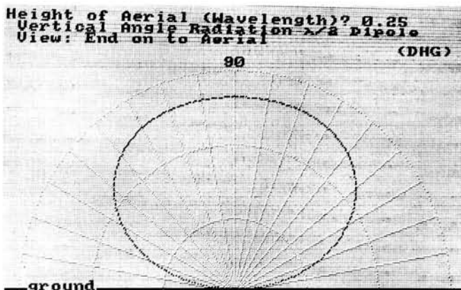
Fig. 1.5: Vertical angle radiation from a half-wave dipole at a height above ground of 0.25 wavelength (see text)
