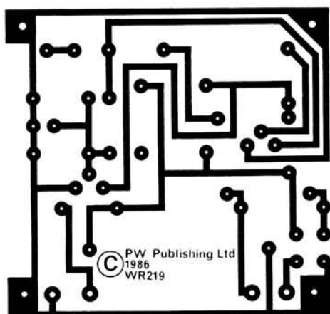
Fig. 6: Track pattern for p.s.u.
