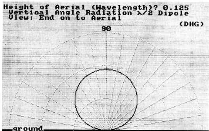
Fig. 1.4: Vertical angle radiation from a half-wave dipole at low height above ground (0.125 wavelength) Note: height in wavelength relative to frequency of operation. Applies to Figs. 1.5, 1.6 and 1.7
