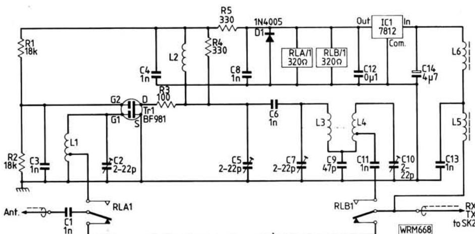
Fig. 1: Circuit diagram of the masthead pre-amp
