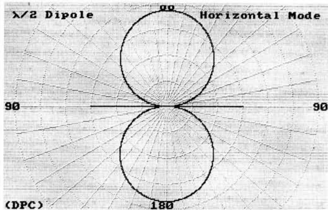
Fig. 1.1: Radiation pattern. Horizontal Dipole. Compare with line diagram of "solid free-space" radiation field as in Fig. 1.2
