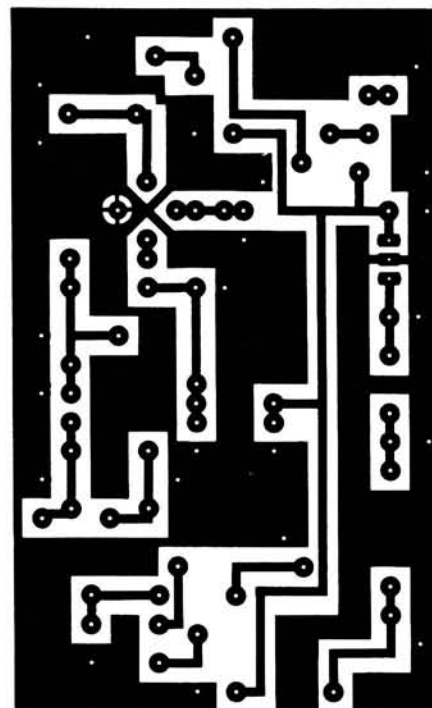
Fig. 3: Track pattern for pre-amp
