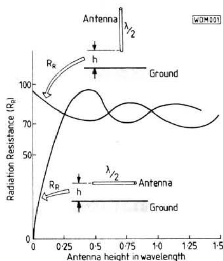
Fig. 1.1: Radiation resistance of both horizontal and vertical half-wave antennas relative to height above ground in wavelength (see text for further explanation)
