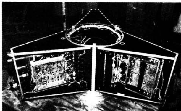
Fig. 1: Phase IIIc and its contents under thermal vacuum tests. From AMSAT-DL
