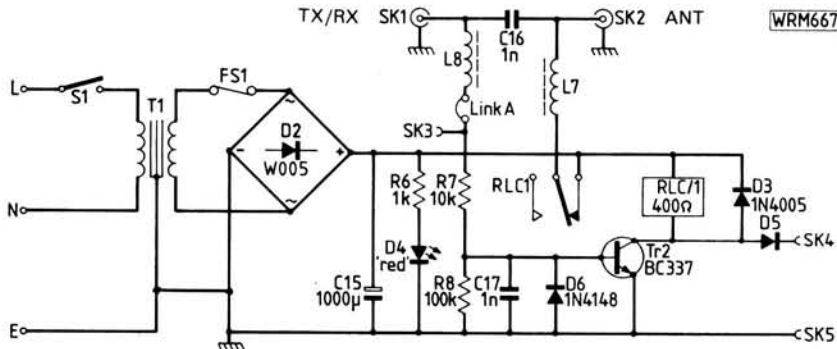
Fig. 2: Circuit diagram of p.s.u. for the masthead pre-amp
